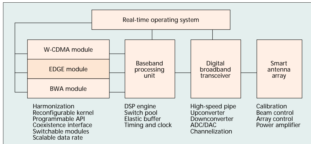
■ Figure 8. Functional segments of the converged broadband wireless systems.
